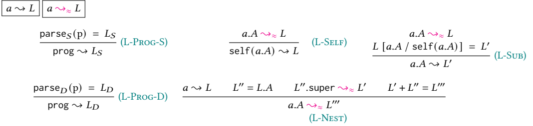
Figure 11. Rules for computing linkages L , parameterized by a program p .
